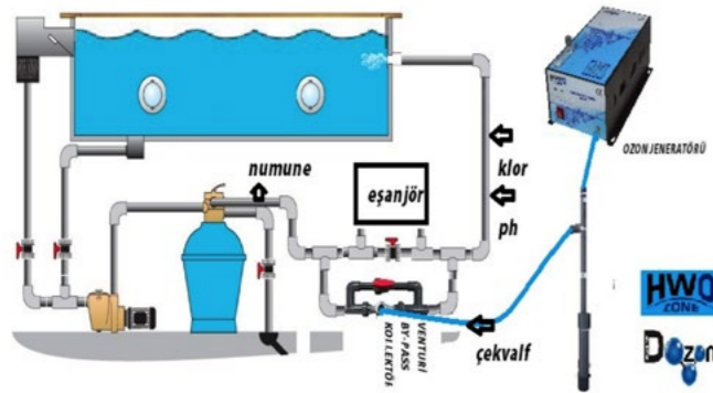
Esvel Havuzlar İçin Venturi By-Pass Montaj Şema Venturi For Domestic Pools By-Pass Installation Diagram
